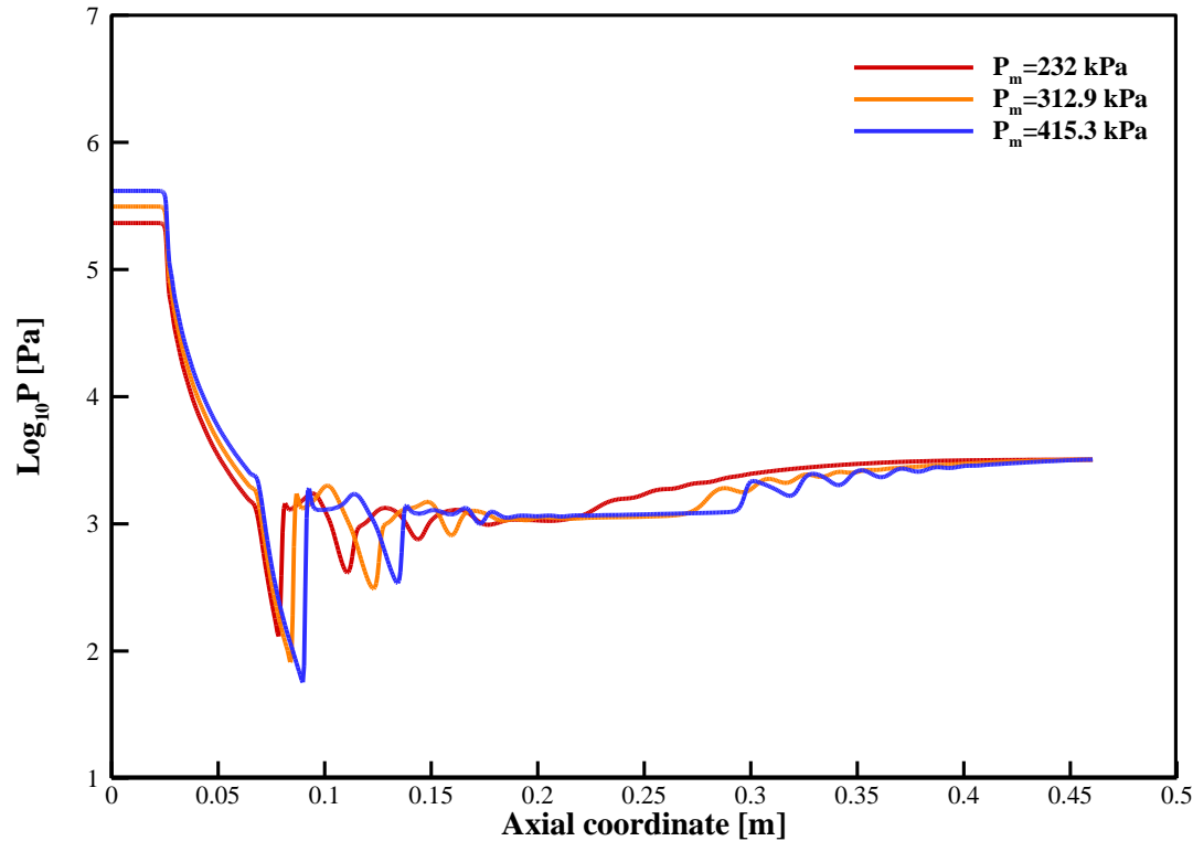
Figure 4. Impact of POMF on the pressure
