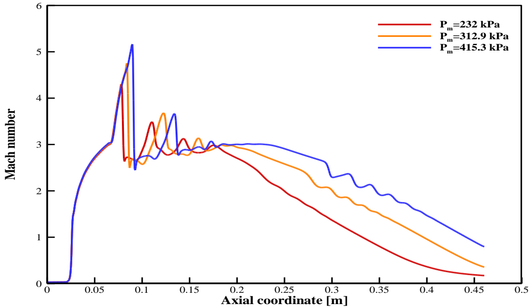
Figure 6. Effect of POMF on the Mach number
