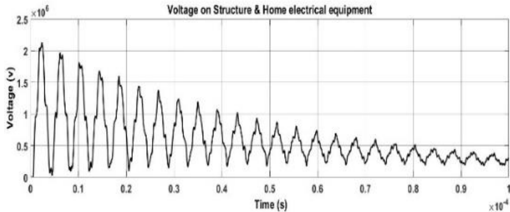
Fig. 11. Voltage waveform on building equipment and structure when lightning strikes middle of the line
