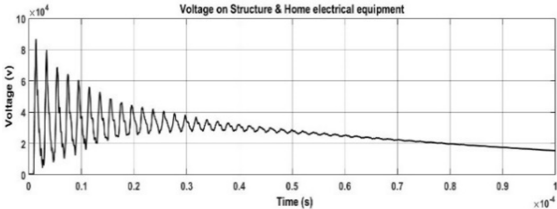
Fig. 14. Voltage waveform on building equipment when lightning strikes at the transformer side
