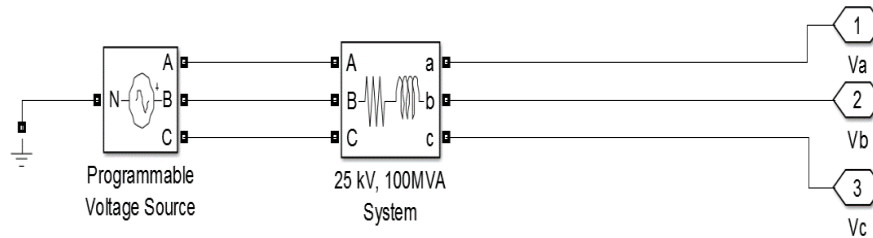
Fig. 3. Simulated source circuit in MATLAB software
